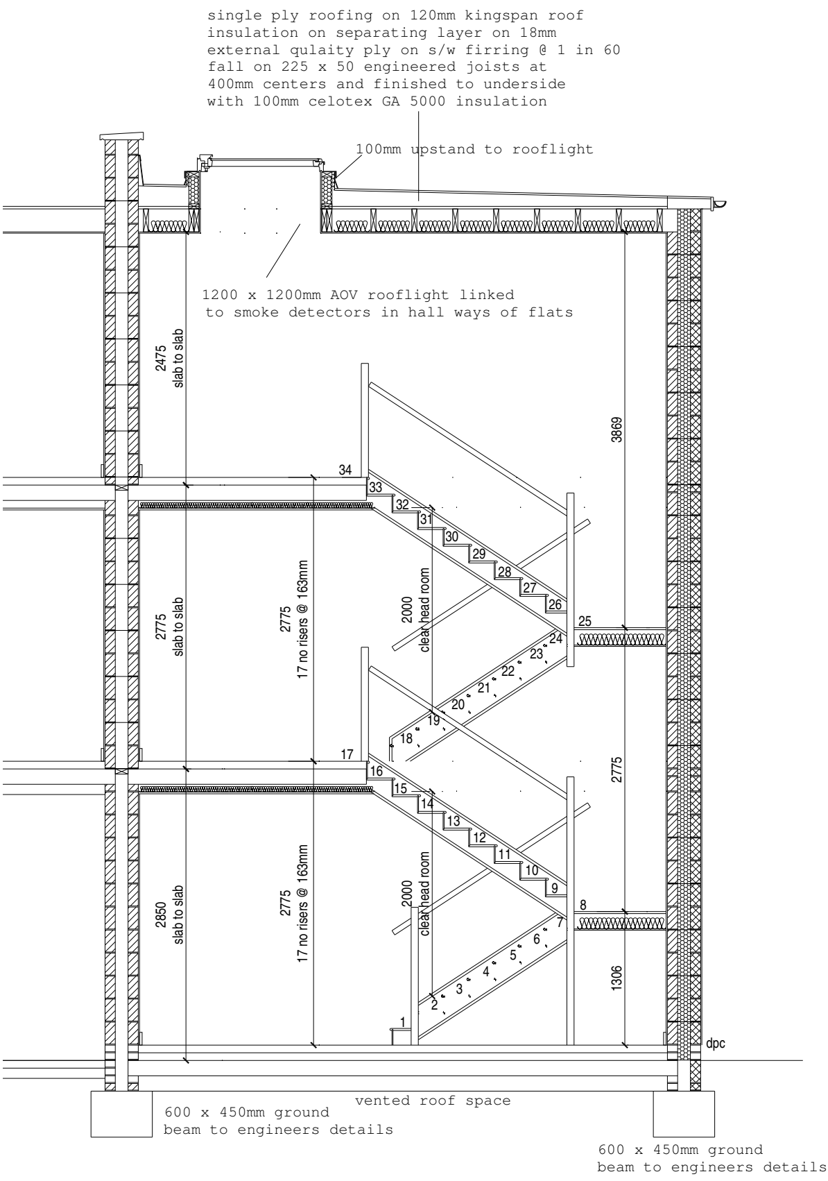
Section F - F
