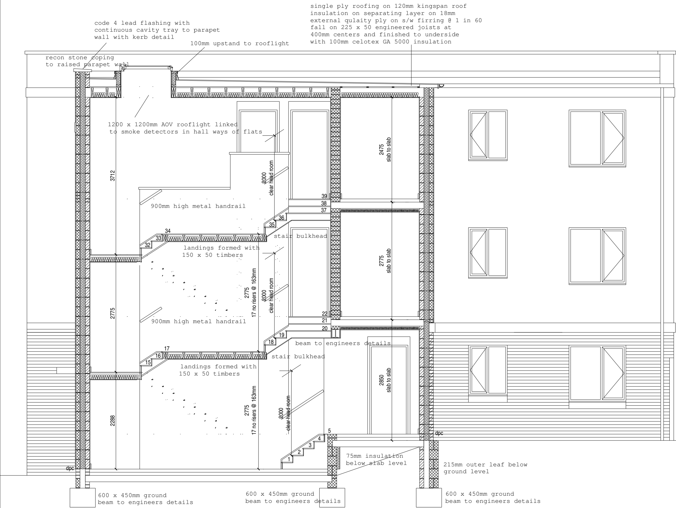
Section C - C
